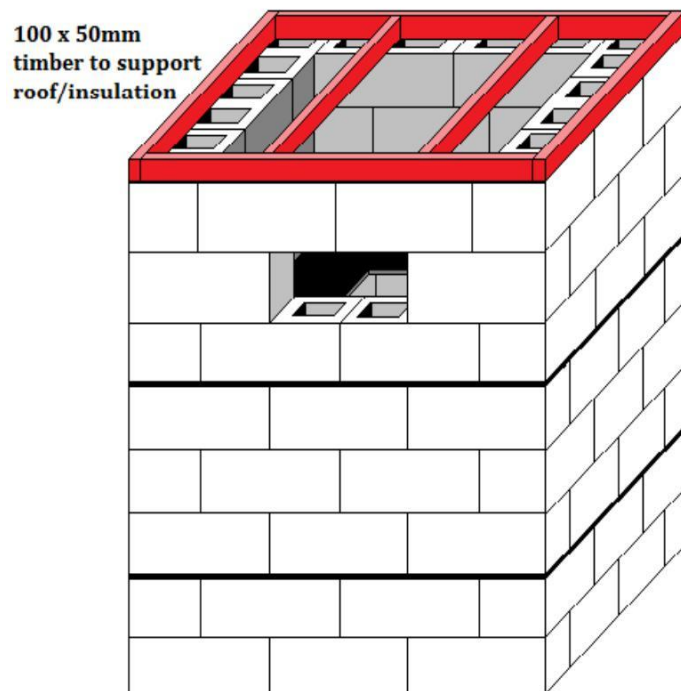
Fig 5. Alternative ceiling/roof support using 100 x 50mm timber.
