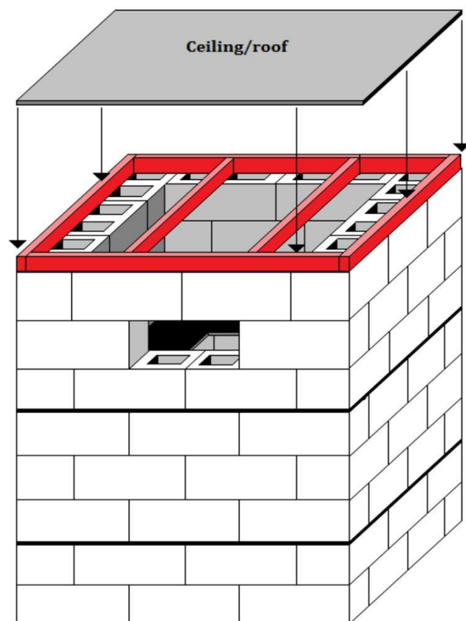
Fig 6: Alternative roof/ceiling construction using 100 x 50mm timbers.
